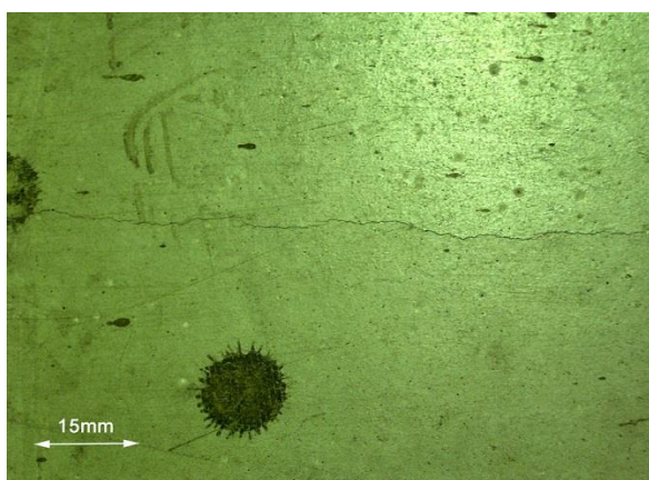
Figure 9. Fine cracked T&G joint. The appearance of the cracks without and with mesh were similar, but the with mesh cracks were much finer. (Note scale is smaller than Fig 8.)
