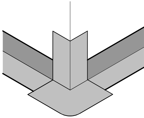
STEP 1 INSTALL EXTERNAL CORNERS BY ADHERING 100MM FLASHING TO THE CORNER AS SHOWN
