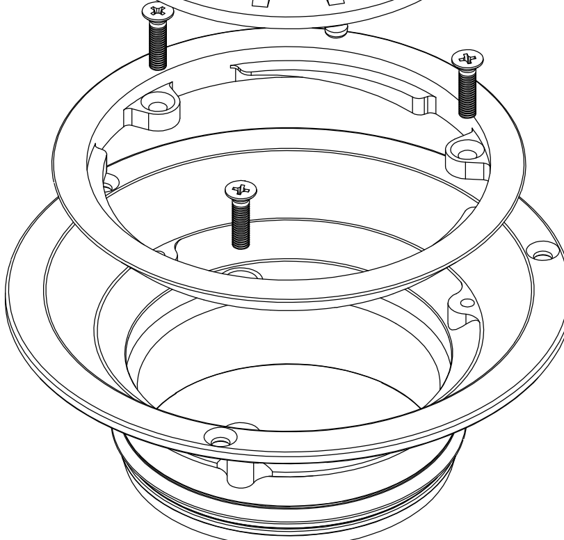
EXPLODED VIEW
