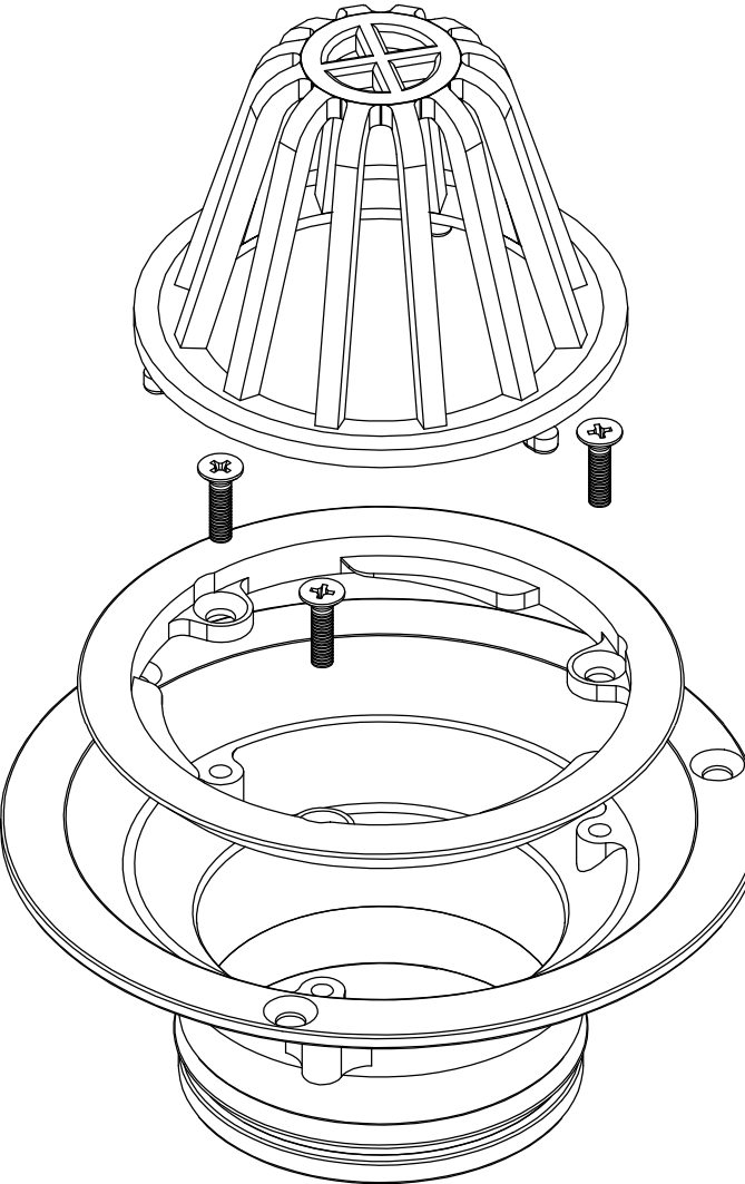
EXPLODED VIEW
